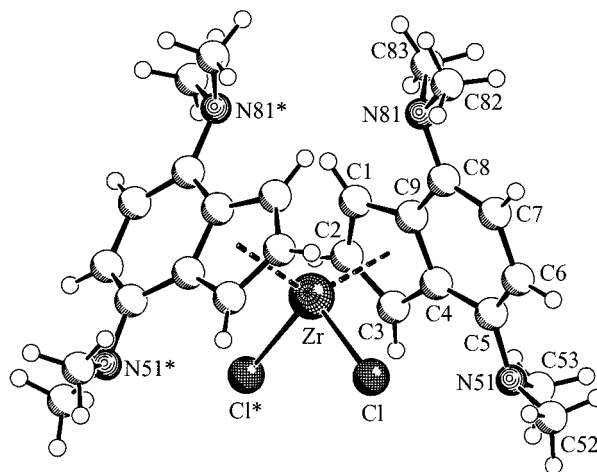
Figure 2. View of the molecular structure of complex 23 (with unsystematic atom-numbering scheme); selected bond lengths [Å] and angles [°]: Zr–Cl 2.417(1), Zr–Cl* 2.467(3), Zr–C2 2.484(3), Zr–C3 2.540(3), Zr–C4 2.639(3), Zr–C9 2.579(3), C1–C2 1.393(5), C1–C9 1.439(4), C2–C3 1.398(5), C3–C4 1.427(5), C4–C9 1.444(4), C8–C9 1.436(4), C4–C5 1.422(4), C8–N81 1.422(4), C5–N51 1.417(4); Cl–Zr–Cl* 98.80(5), C1–C2–C3 109.9(3), C2–C1–C9 107.6(3), C2–C3–C4 108.3(3), C1–C9–C8 132.9(3), C3–C4–C5 132.0(3), C9–C8–N81 119.0(3), C4–C5–N51 118.0(3).
