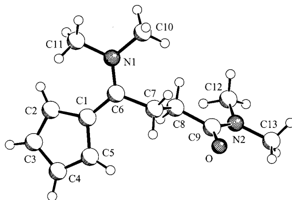
Figure 1. View of the carboxamide-functionalized aminopentafulvene system 16 ; selected bond lengths [Å] and angles ^\circ : C1–C2 1.450(2), C2–C3 1.355(3), C3–C4 1.421(3), C4–C5 1.357(3), C5–C1 1.438(3), C1–C6 1.399(2), C6–N1 1.337(2), C6–C7 1.511(2), C7–C8 1.527(2), C8–C9 1.515(2), C9–O 1.222(2), C9–N2 1.349(2); C2–C1–C5 105.1(2), C2–C1–C6 130.1(2), C5–C1–C6 124.7(2), C1–C6–N1 124.9(2), C1–C6–N7 118.3(2), N1–C6–C7 116.8(2), C6–C7–C8 112.1(1), C7–C8–C9 111.5(1), C8–C9–O 120.9(1), C8–C9–N2 117.0(2), O–C9–N2 122.1(2).
