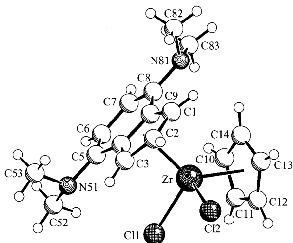
Figure 3. Molecular structure of complex 24 ; selected bond lengths [Å] and angles [°]: Zr–Cl1 2.440(1), Zr–Cl2 2.441(1), Zr–C1 2.477(2), Zr–C2 2.508(2), Zr–C3 2.527(2), Zr–C4 2.601(2), Zr–C9 2.577(2), Zr–C10 2.494(2), Zr–C11 2.537(2), Zr–C12 2.514(2), Zr–C13 2.483(2), Zr–C14 2.492(2), C1–C2 1.404(3), C1–C9 1.440(3), C2–C3 1.403(3), C3–C4 1.439(3), C4–C9 1.438(3), C8–C9 1.433(3), C4–C5 1.427(3), C8–N81 1.411(3), C5–N51 1.421(3), Cl1–Zr–Cl2 96.98(2), C1–C2–C3 109.9(2), C2–C1–C9 107.5(2), C2–C3–C4 107.6(2), C1–C9–C8 132.4(2), C3–C4–C5 131.5(2), C9–C8–N81 118.7(2), C4–C5–N51 118.1(2)
